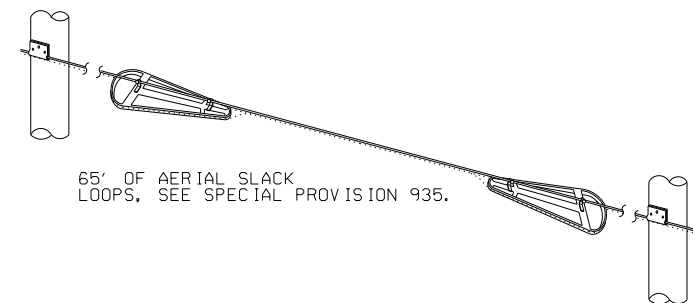
AERIAL SLACK LOOP DETAIL
