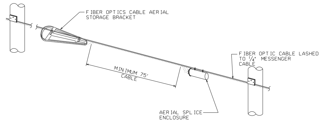
AERIAL BUTT SPLICE DETAIL
