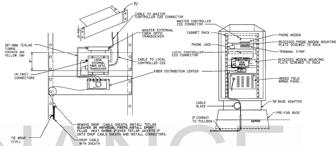
FIBER OPTIC DETAIL DROP - CABLE TERMINATION IN CONTROL CABINET MODEL 332 - MASTER SYSTEM
