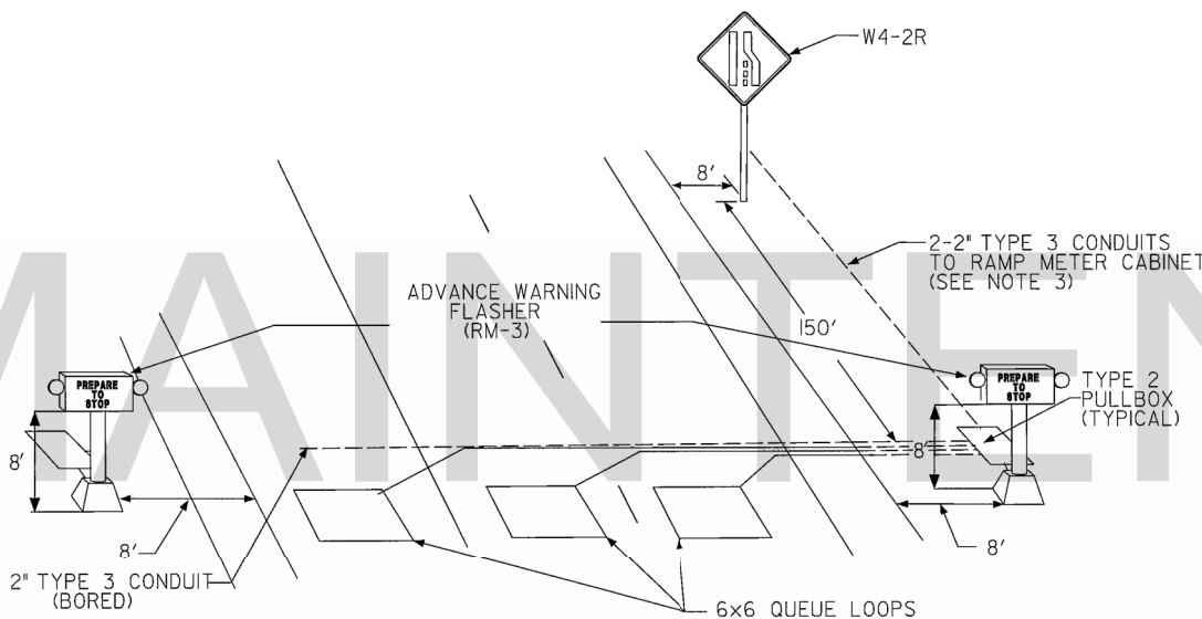
QUEUE LOOP AND ADVANCE WARNING FLASHER PLACEMENT TRIPLE LANE
