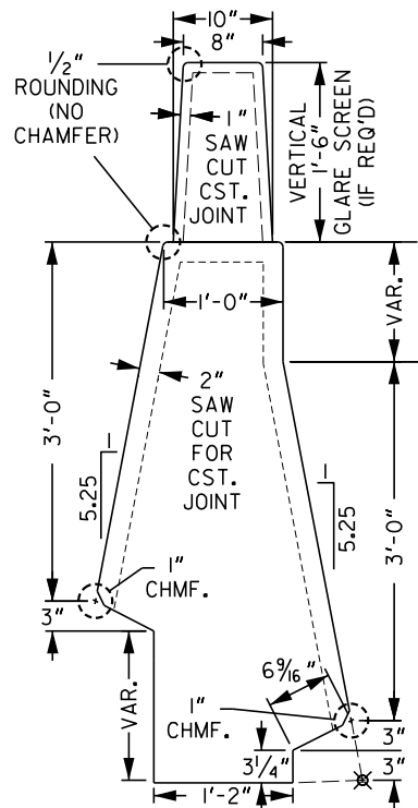
MODIFIED CONCRETE BARRIER DIMENSION DETAIL
