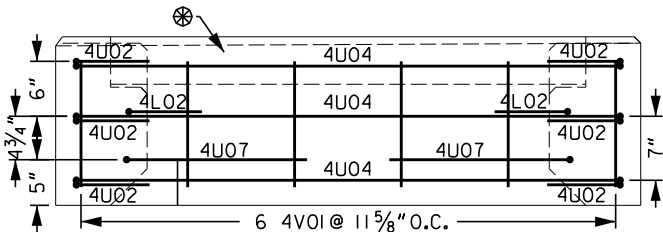
SECTION F-F
