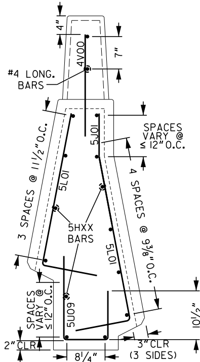
MODIFIED CONCRETE BARRIER TRANSVERSE REINFORCEMENT DETAIL (6" O.C.)
