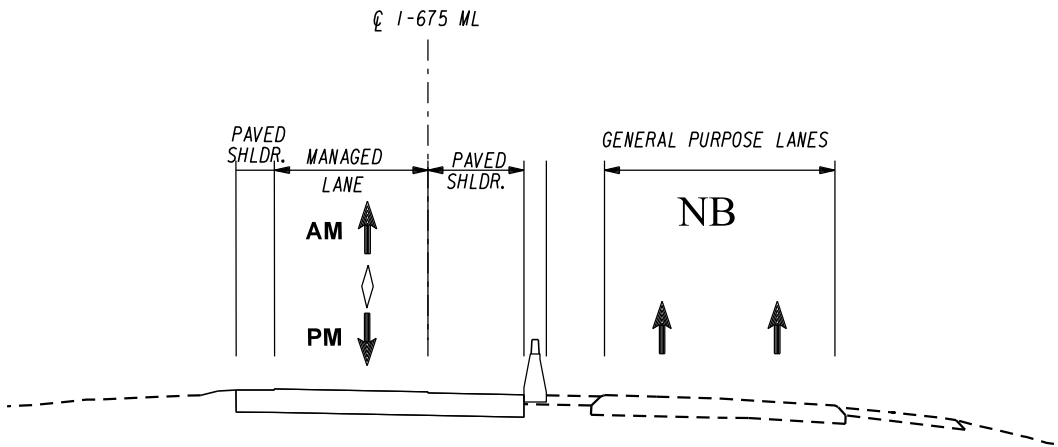
CONSTRUCTION STAGE 2
