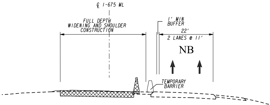
CONSTRUCTION STAGE 1
