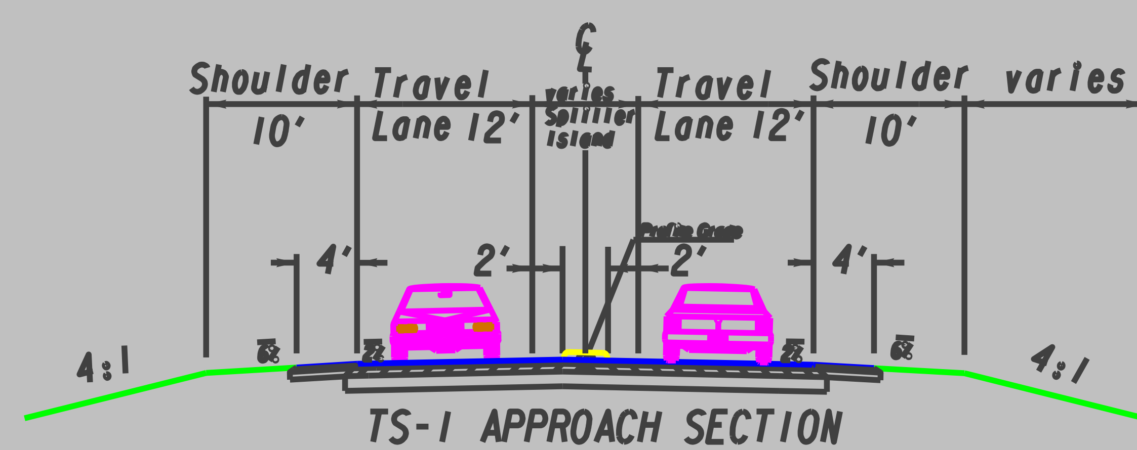
TYPICAL SECTIONS
