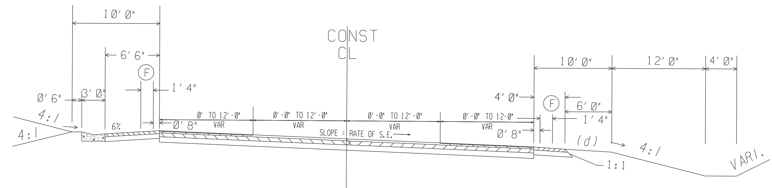
TYPICAL SECTION
