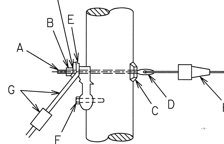
DETAIL "A" (SEE PARTS LIST)
