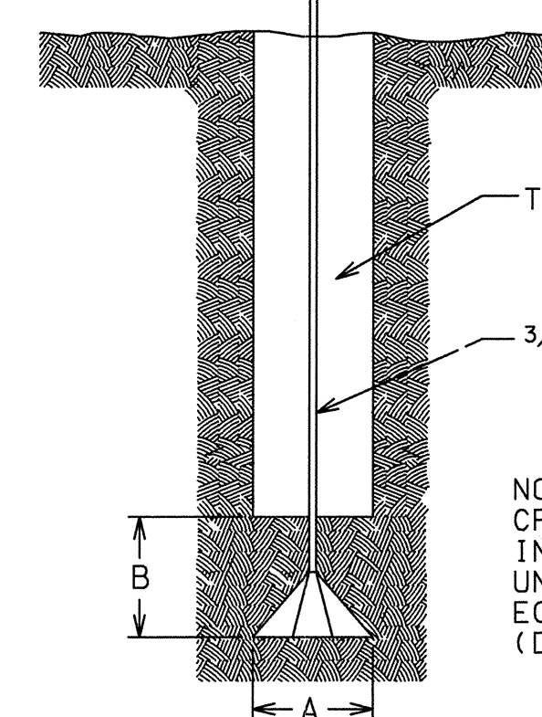
DETAIL "C"
