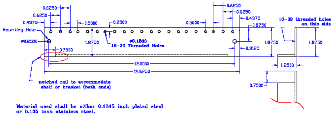
DETAIL C - EIA Angle Rail w/ EIA universal hole spacing Refer to EIA-310-B
