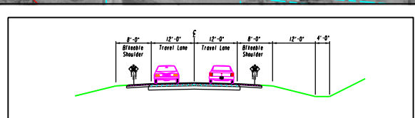
TYPICAL SECTION: SOUTH TIFTON BYPASS FROM UNION ROAD TO TECH DRIVE (45 MPH)
