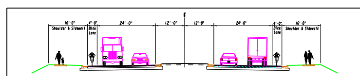
TYPICAL SECTION: SOUTH TIFTON BYPASS FROM TECH DRIVE TO MAGNOLIA INDUSTRIAL BLVD (45 MPH)
