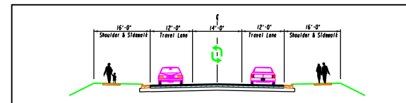
TYPICAL SECTION: SOUTH TIFTON BYPASS FROM MAGNOLIA INDUSTRIAL BLVD TO SR 125 (45 MPH)
