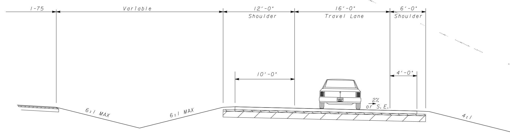
Ramp Typical Section
