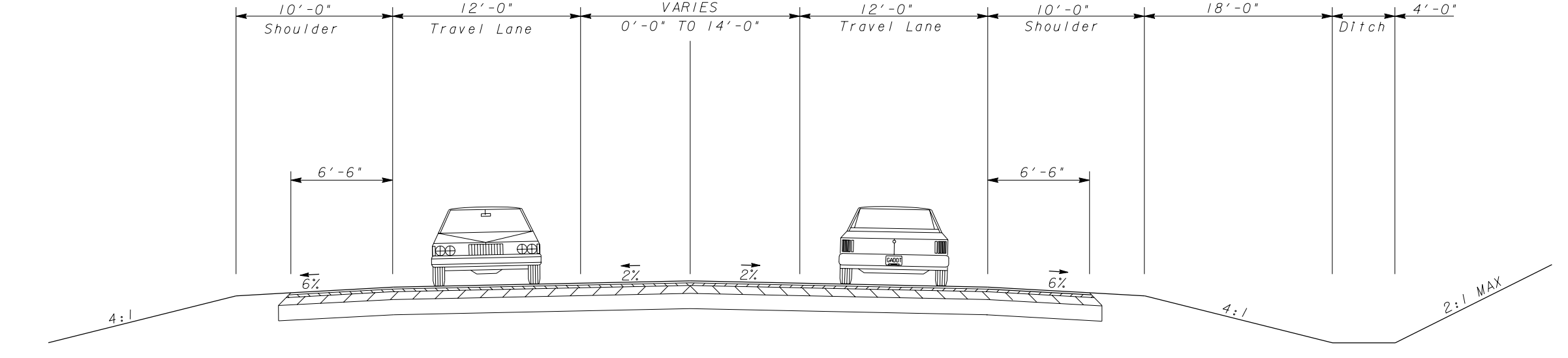
Typical Section at Chula Brookfield Road
