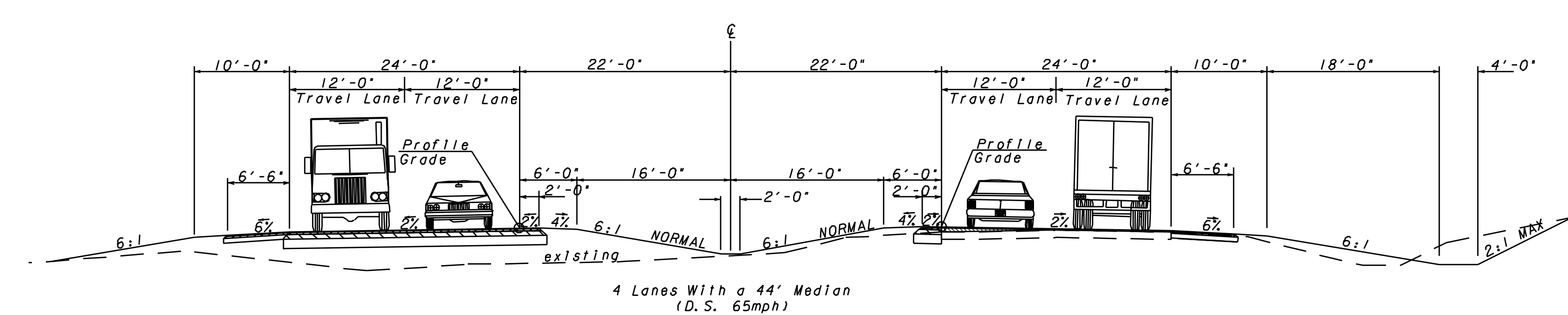
TYPICAL SECTION
