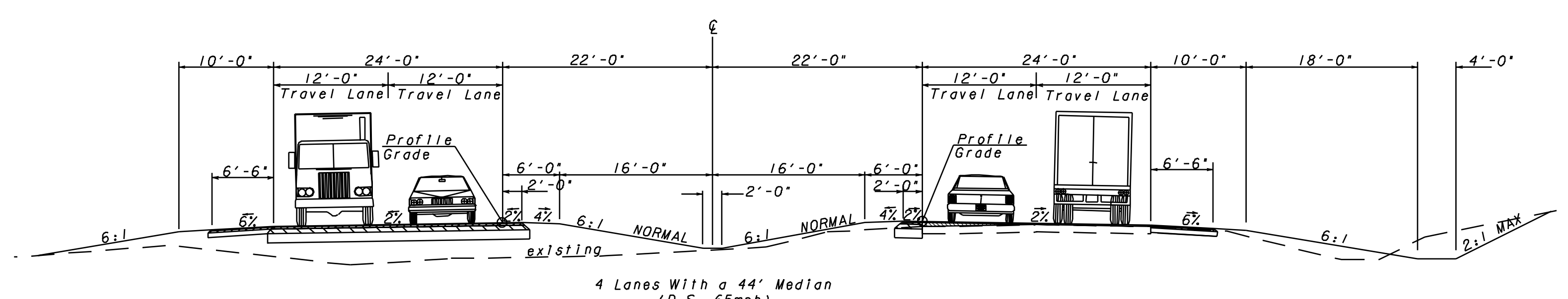
TYPICAL SECTION
