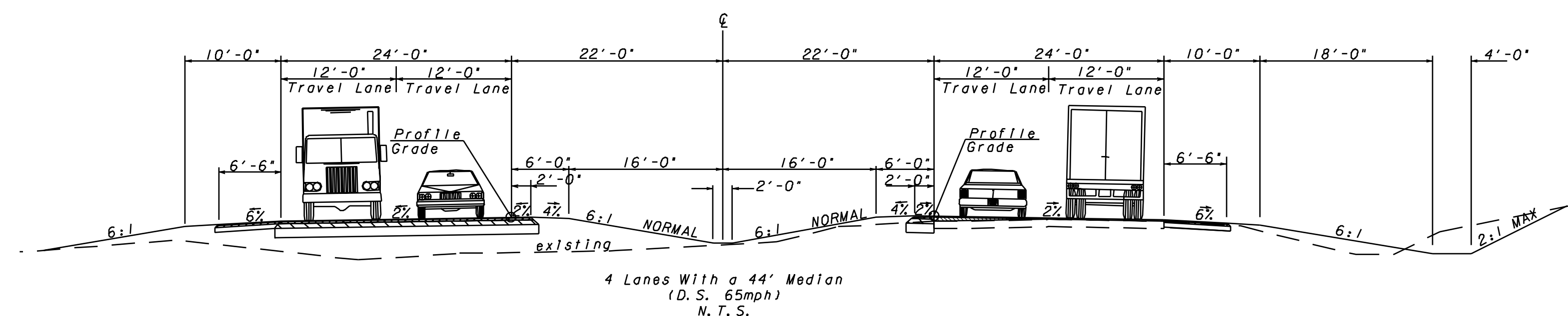
TYPICAL SECTION
