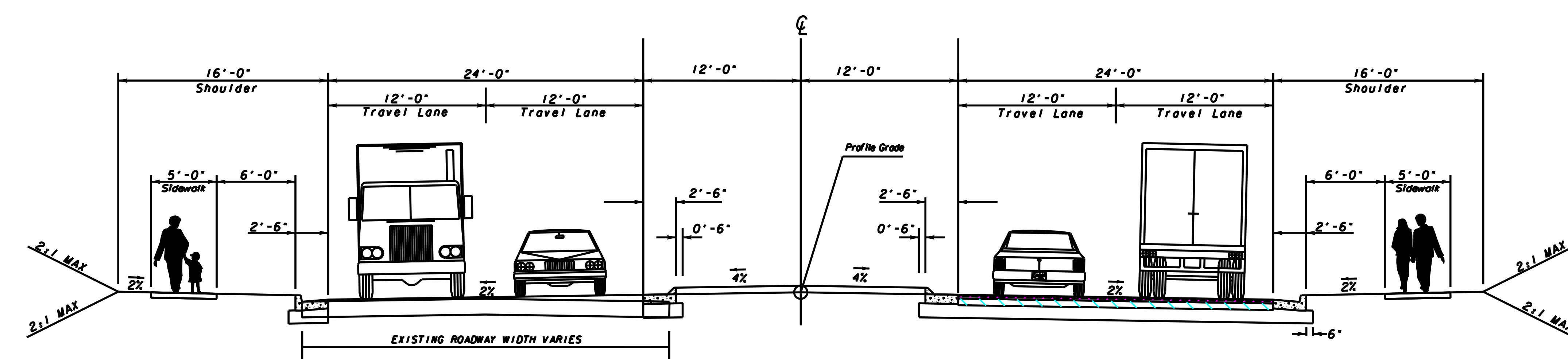
24' RAISED MEDIAN
